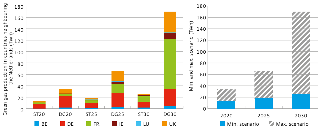
FIGURE 2.17 GREEN GAS PRODUCTION IN COUNTRIES NEIGHBOURING THE NETHERLANDS UNDER THE ENTSOG SCENARIOS.
